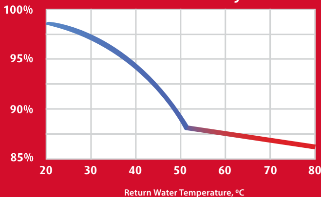
Boiler Efficiency
