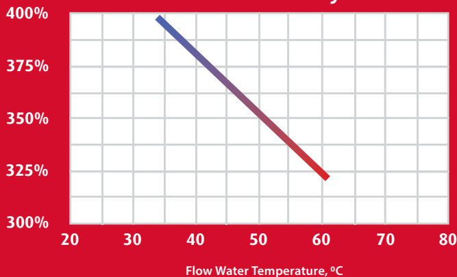
ASHP Efficiency
